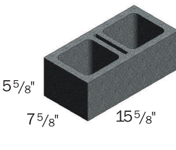
6-inch High Splitable
