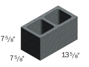
14-inch Long
