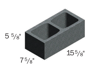
6-inch High
