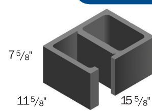
Inspection
