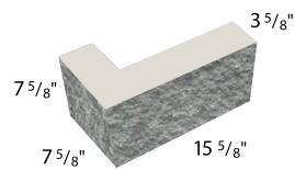
4-inch L-Corner
