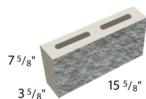
4-inch Regular
