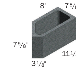
Single 45
