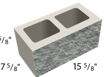
8-inch Regular
