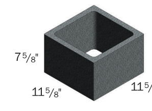
Column (C-12)
