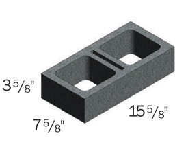
Half High Splitable
