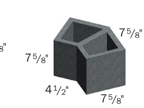
Double 45
