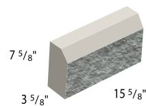
4-inch Sill (8 High)
