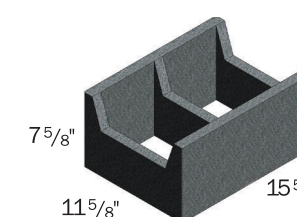
Bond Beam
