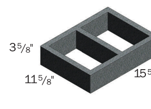
12-Inch Half High
