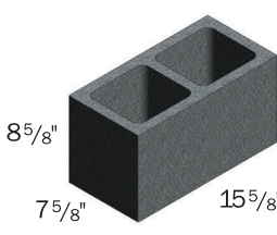
9-inch High
