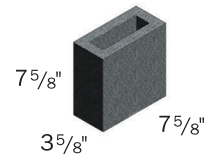
Half Partition
