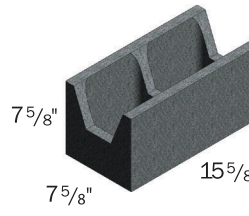
Bond Beam
