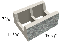
12-inch Bond Beam
