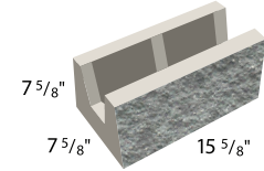
8-inch Bond Beam
