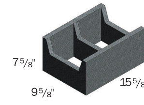
Bond Beam
